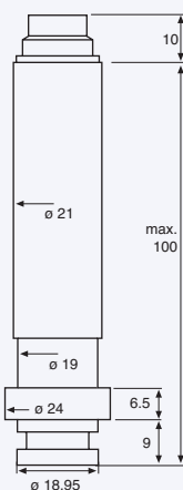
Series 35 X HT (Manometer Pressure Port)
